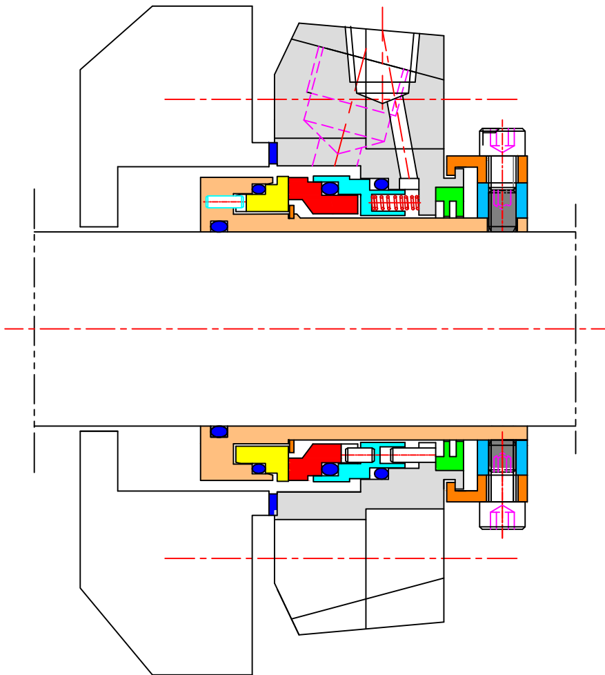
90 SERIES MULTI SPRINGS BALANCED SLURRY MECHANICAL SEAL TYPE 9902 CARTRIDGE ARRANGEMENT WITH DIFFERENT API PLAN 11& 62
